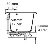
Section BB Shown with K31 Waste Kit
